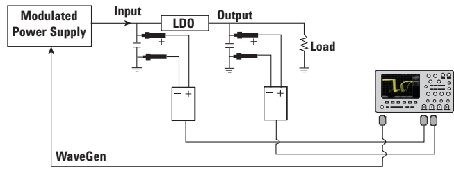
Figure 9. The PSRR is defined as the ratio of the output ripple compared to the input ripple over a wide frequency range.
